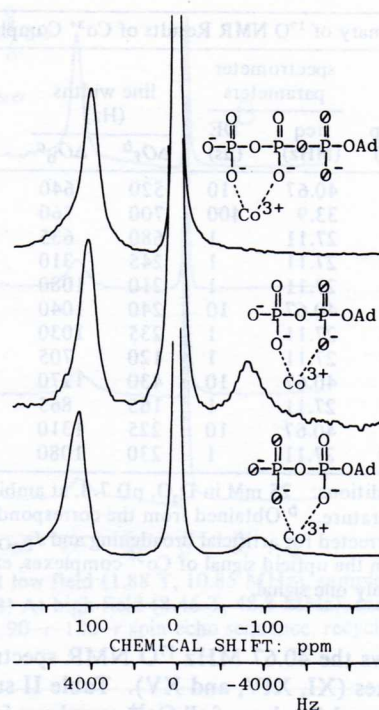
FIGURE 4: ^{17}O NMR spectra of the Co^{3+} complexes XI, XIV, and XV at 40.67 MHz. Sample conditions and spectrometer conditions are same as those of Figure 2.
