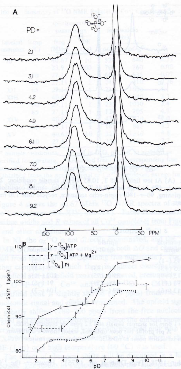
FIGURE 7: (A) Low-field (1.88 T, 10.85 MHz) ^{17}\text{O} NMR spectra of [\text{O}_4]^{17}\text{P}_i at various pD. Sample condition: 25 mM in \text{D}_2\text{O} , with pD adjusted by DCl and NaOH; EDTA 2 mM. Spectrometer (Varian FT-80) condition: spectral width 8 kHz, 1.6 K data points, DE = 200 \mu\text{s} , deuterium lock, recycle time 120 ms, 20 000 transients. (B) Plot of chemical shifts vs. pD for [\text{O}_4]^{17}\text{P}_i [from the spectra in (A)] and [\gamma\text{-}^{17}\text{O}_3]\text{ATP} (III) and \text{Mg}^{2+}/[\gamma\text{-}^{17}\text{O}_3]\text{ATP} at medium field (4.7 T, 27.11 MHz). Sample conditions for ATP: 25 mM in \text{D}_2\text{O} , EDTA 1 mM. Spectrometer parameters (Bruker WP-200): 2K data points, spectral width 20 kHz, DE = 12 \mu\text{s} , deuterium lock, recycle time 60 ms, line broadening 40 Hz, 15 000 transients. The chemical shift is taken at the center of each peak.
