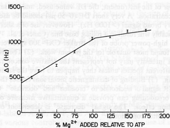
FIGURE 1: ^{17}\text{O} line widths of [\gamma\text{-}^{17}\text{O}_3]\text{ATP} (III) as a function of \text{Mg}(\text{NO}_3)_2 concentration at low field (1.88 T, 10.85 MHz). Sample condition: 25 mM in \text{D}_2\text{O} , pD 7.6. Spectrometer (Varian FT-80) condition: 1K data points, sweep width 8 KHz, DE = 200 \mu\text{s} , deuterium lock, recycle time 120 ms, line broadening 10 Hz. The spectra of this experiment are shown in Figure 5B. The \Delta\text{O} in the plot has not been corrected for exponential multiplication and J_{\text{P-O}} .
