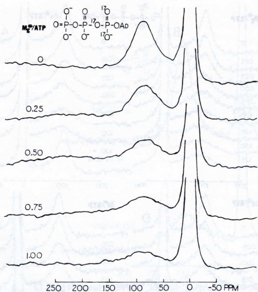
FIGURE 3: Effect of Mg^{2+} on the ^{17}O NMR spectra of [\alpha\text{-}^{17}O_2, \alpha\beta\text{-}^{17}O]ATP (I) in a low magnetic field (2.11 T, 12.2 MHz). Sample condition: 100 mM in D_2O , pD 7.6. Spectrometer (JEOL FX-90Q) condition: Sweep width 10 kHz, 1 K data points, DE = 50.5 \mu s , deuterium lock, line broadening 10 Hz, recycle time 160 ms, 10000 transients. The sharper peak at -3 ppm is due to solvent.
